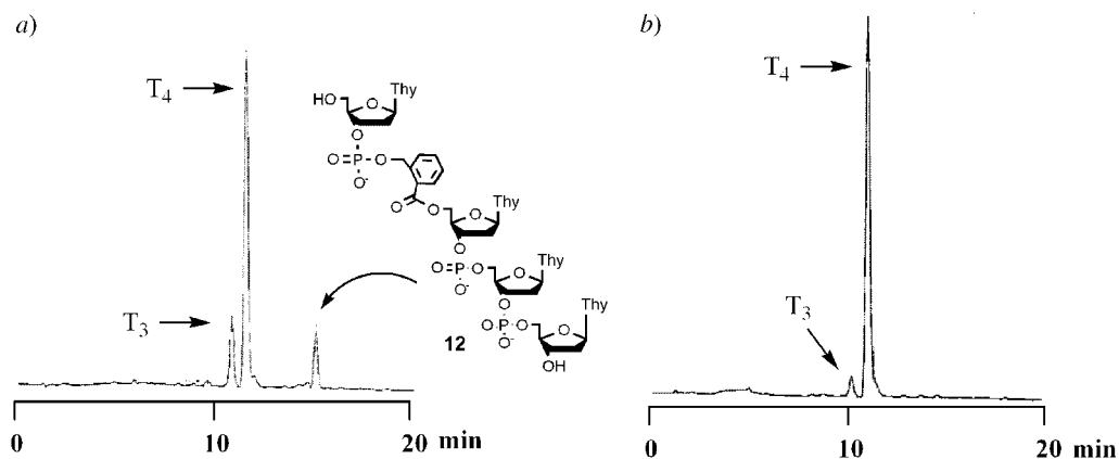
Fig. 1. Reversed-phase HPLC profiles of T_4 synthesized by a combination of conventional (MeO)_2Tr -phosphoramidite and MOB-phosphoramidite 11 for a time period of a) 1 min and b) 5 min for Step 3b in Scheme 8, resp.
